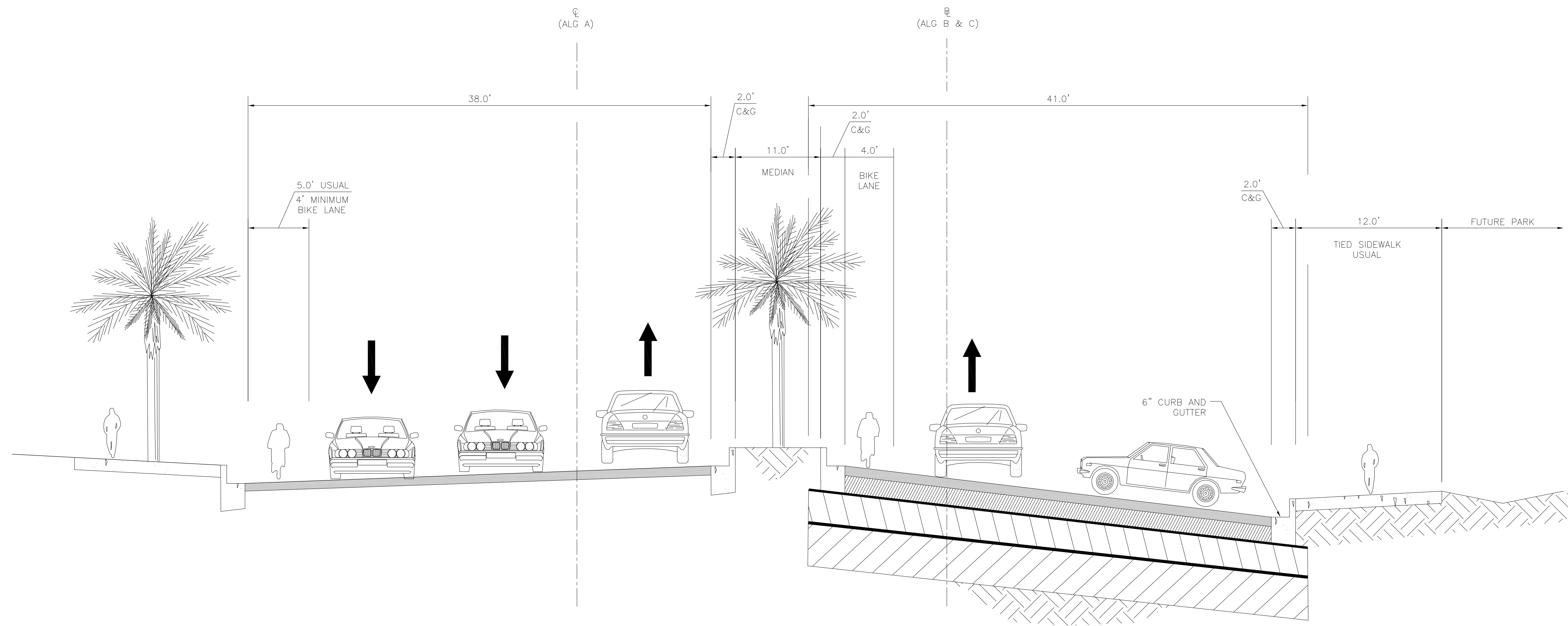
SHORELINE BOULEVARD PROPOSED ROAD SECTION A-A SCALE: N.T.S.
