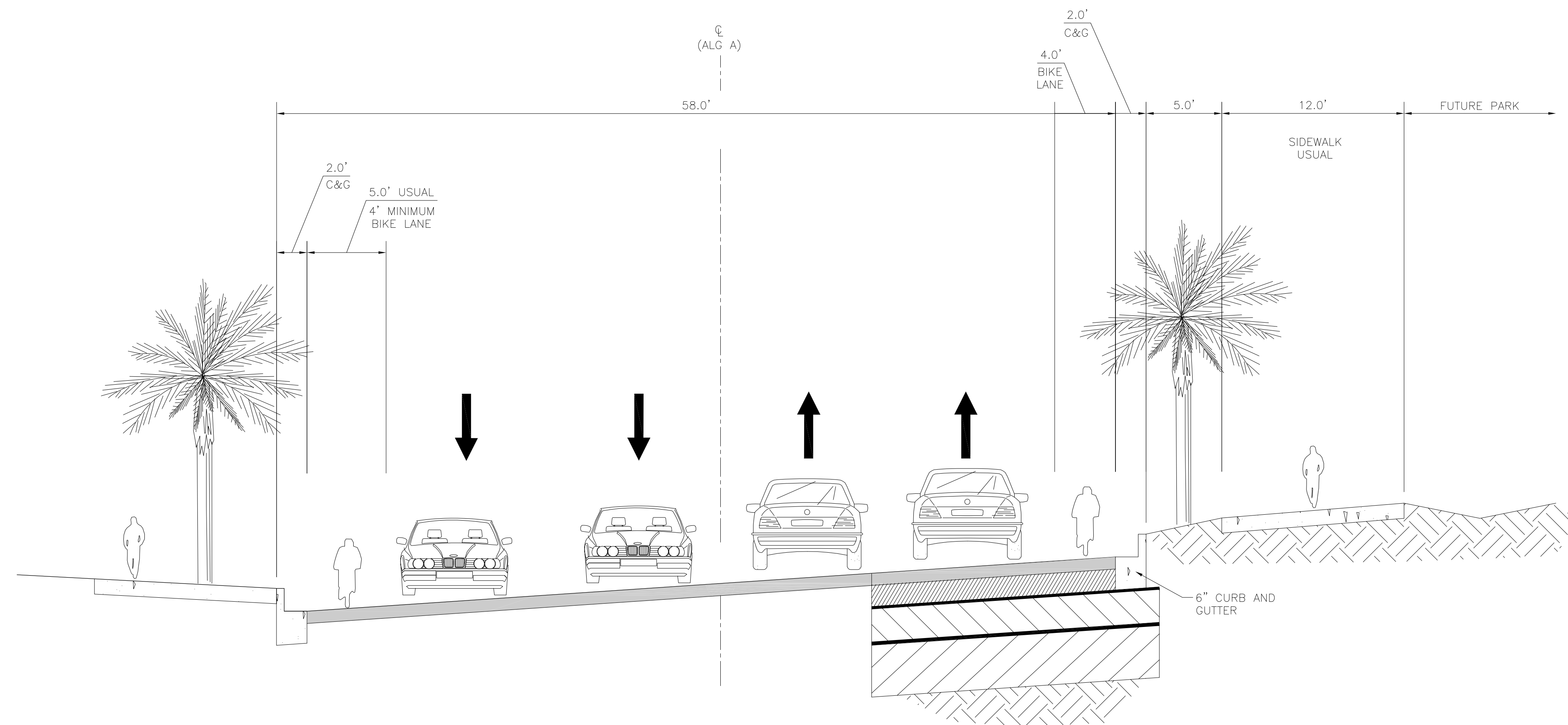
SHORELINE BOULEVARD PROPOSED ROAD SECTION B-B SCALE: N.T.S.
